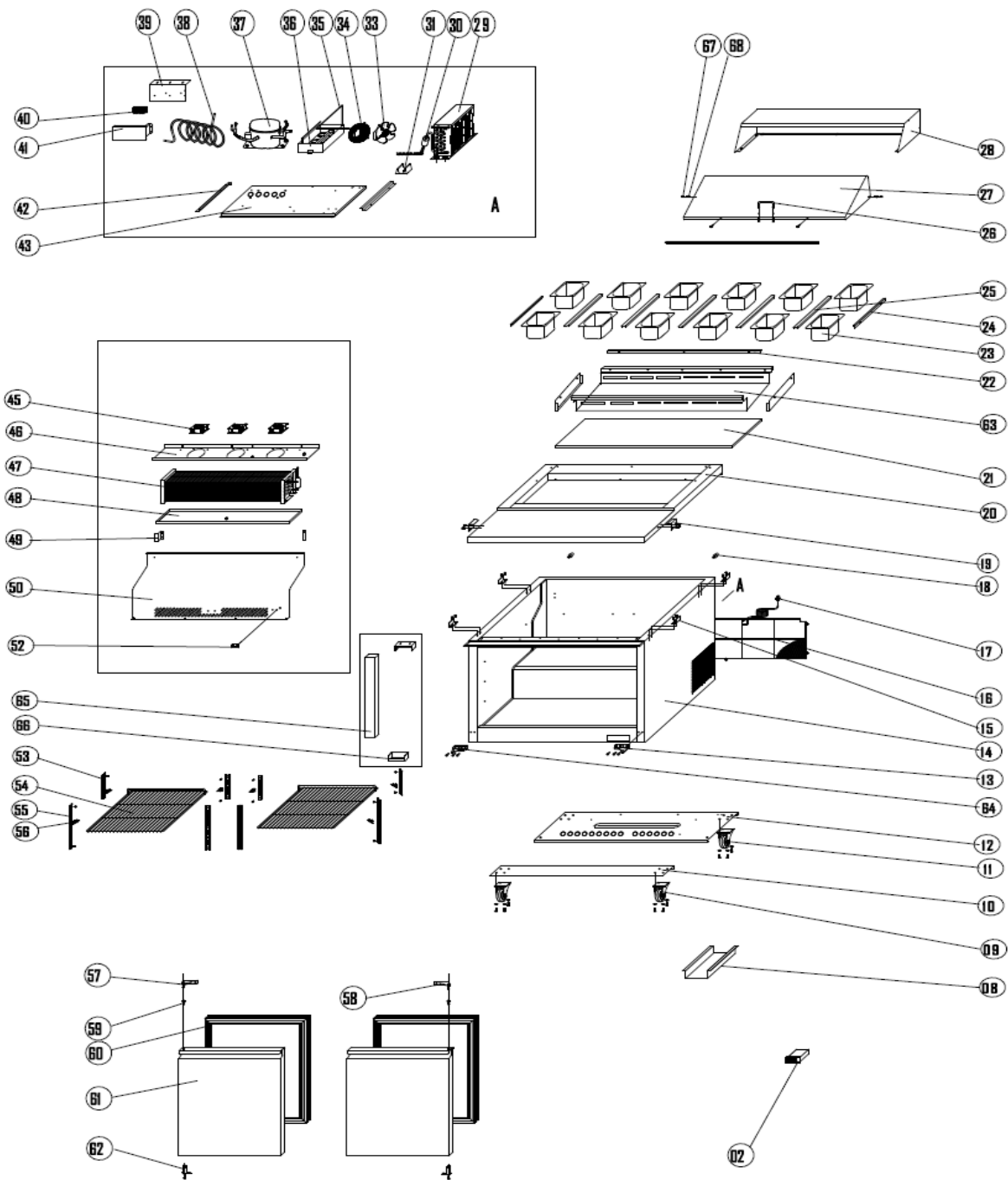
EXPLODE OF KCHST48.12
